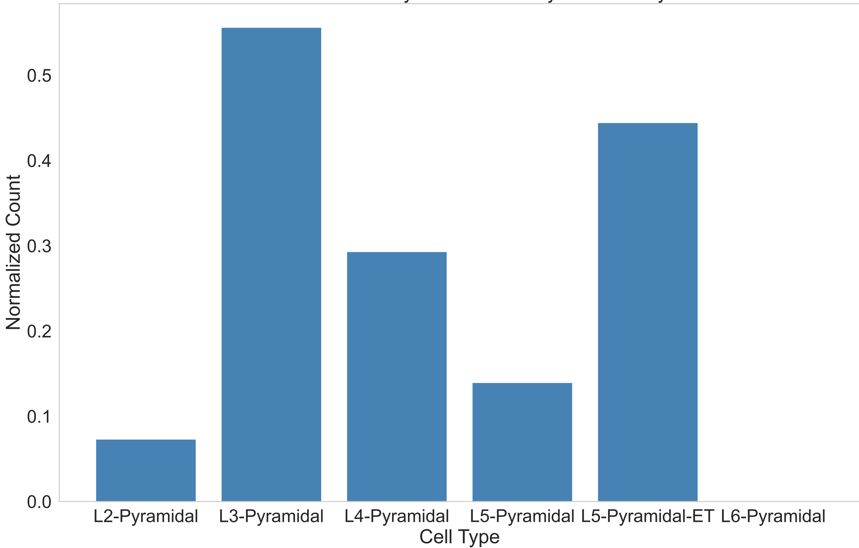
Inbound Excitatory — No Assembly to Assembly
